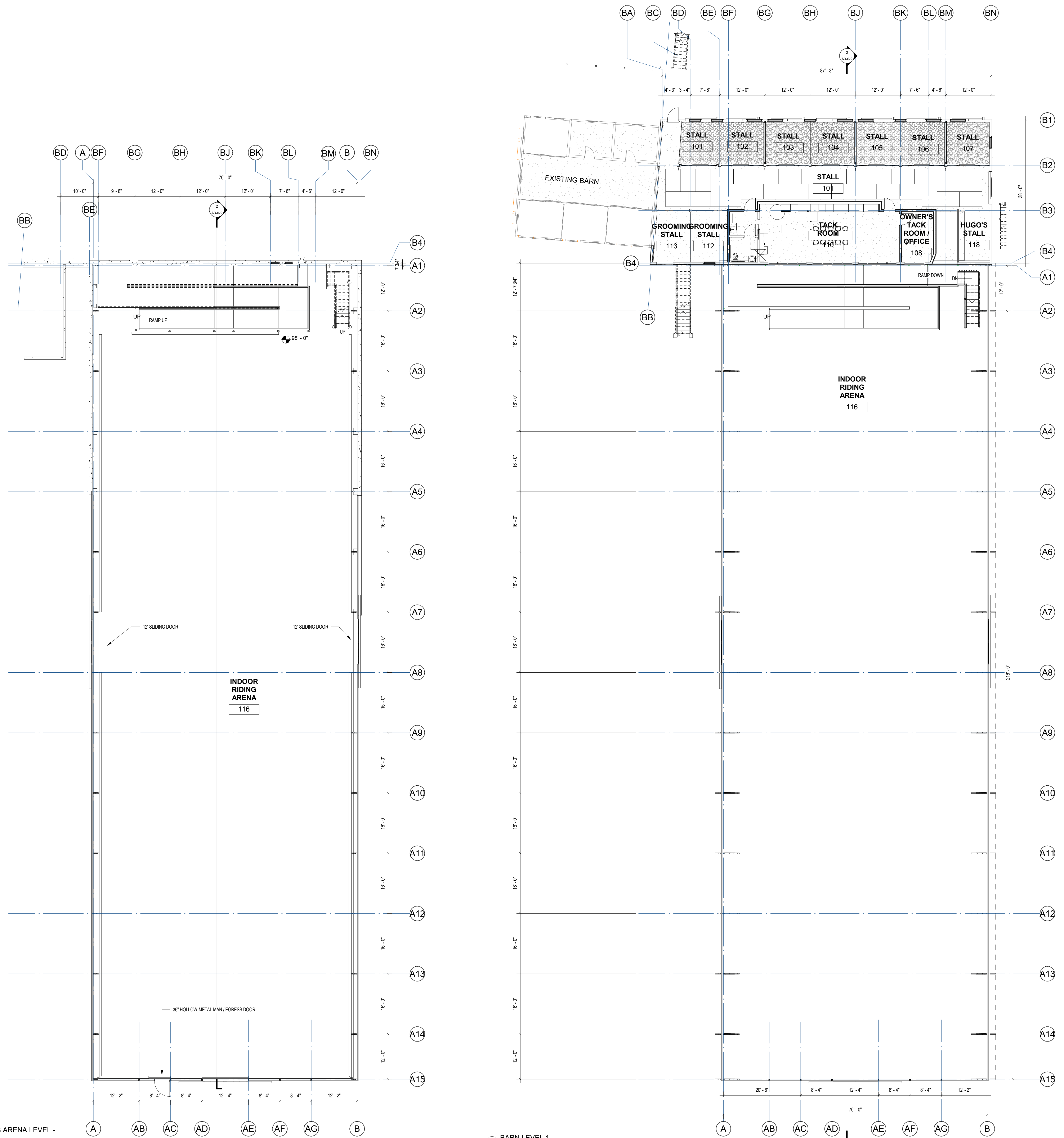
1 BARN LEVEL 1 3/32" = 1'-0"
